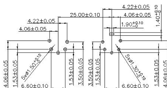
PCB cut-out size PCB 开孔尺寸
