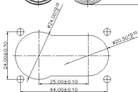
Panel cut-out size 面板开孔尺寸
