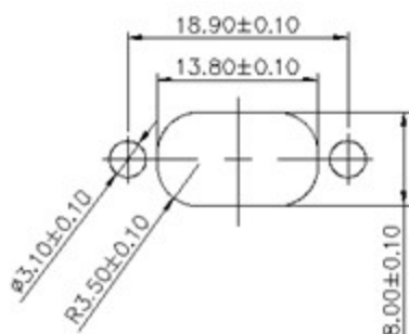
Mounting cut-out size 安装开孔尺寸
